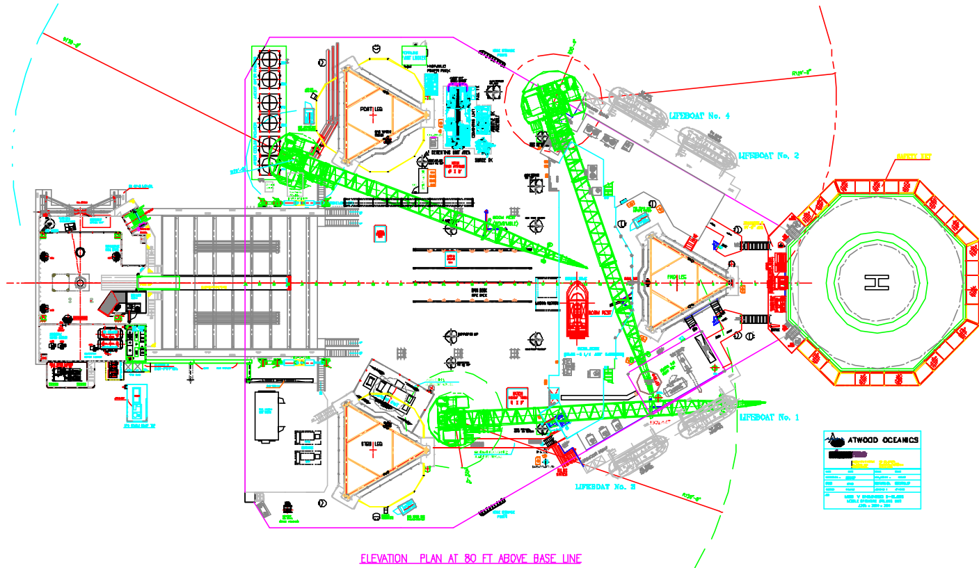
ELEVATION PLAN AT 80 FT ABOVE BASE LINE
